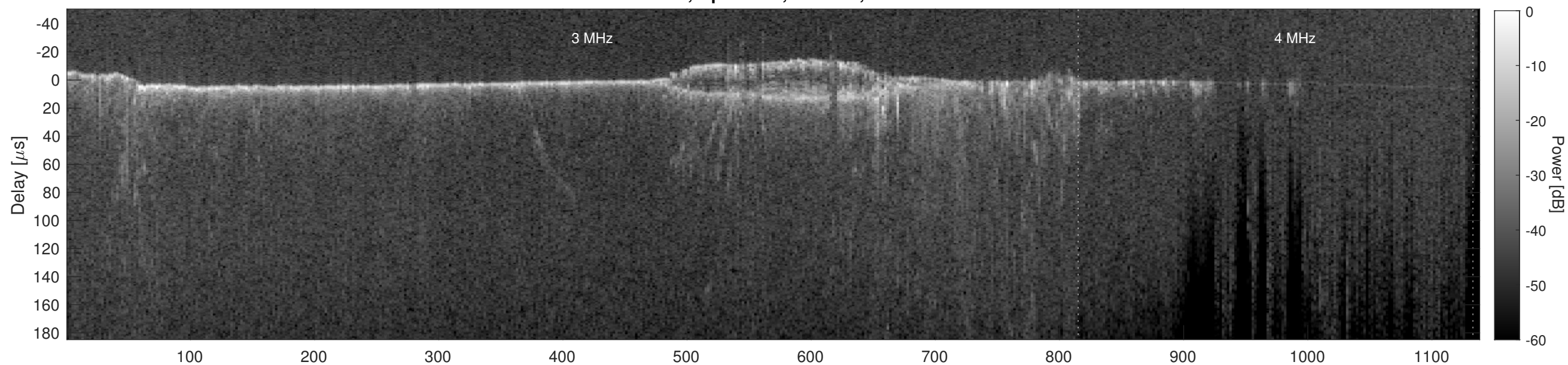
Orbit 11905, Cluttergram
