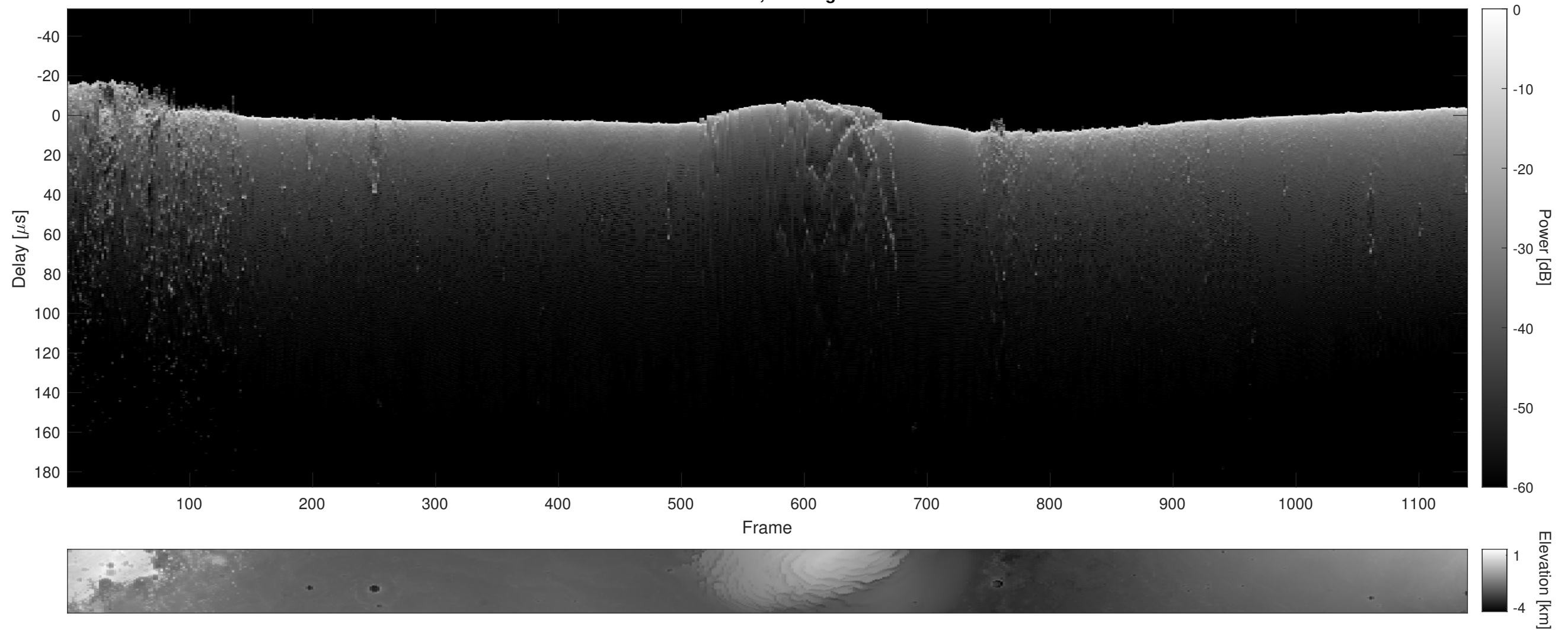
Orbit 11908, Cluttergram
