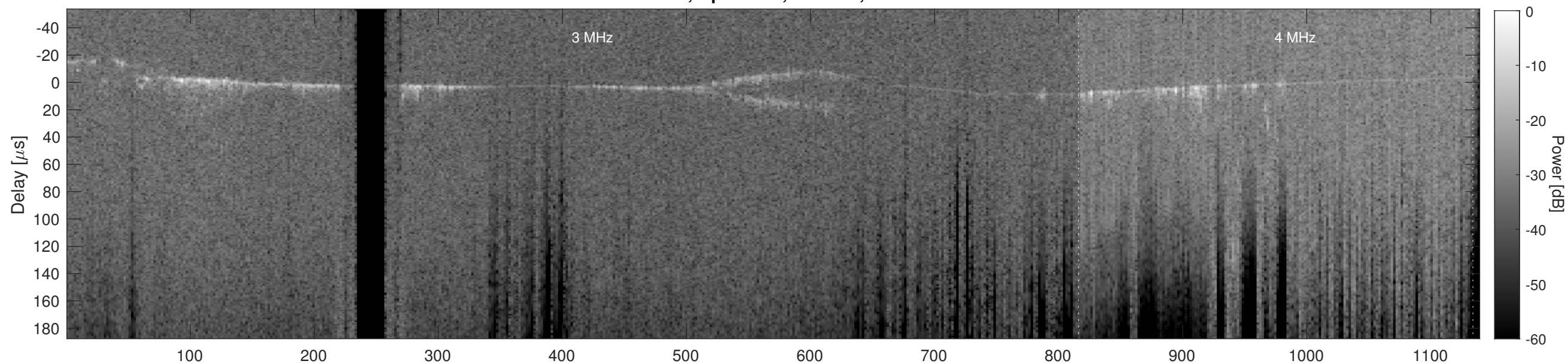
Orbit 11908, Cluttergram
