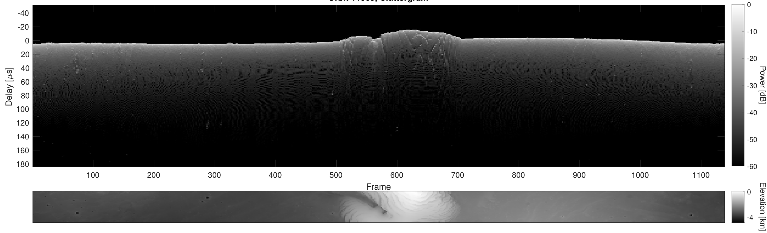
Orbit 11909, Cluttergram
