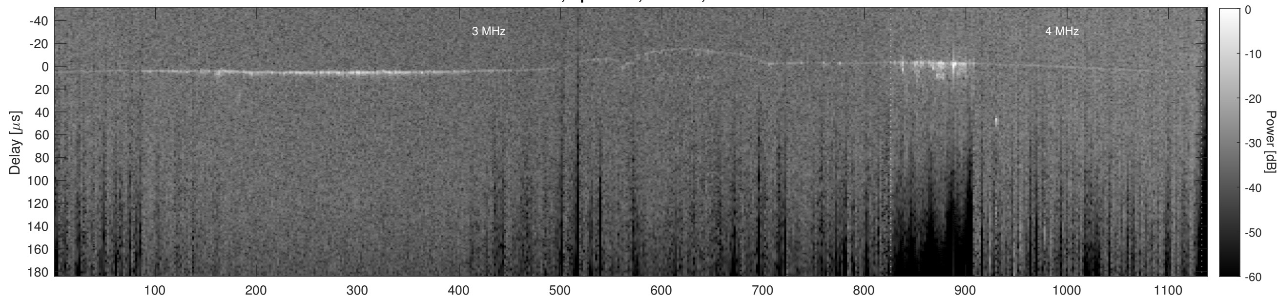
Orbit 11909, Cluttergram
