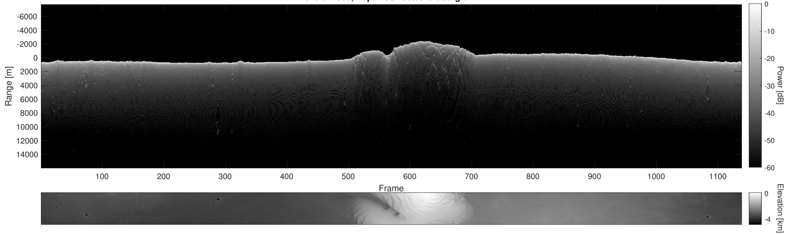
Orbit 11909, Depth-Corrected Cluttergram
