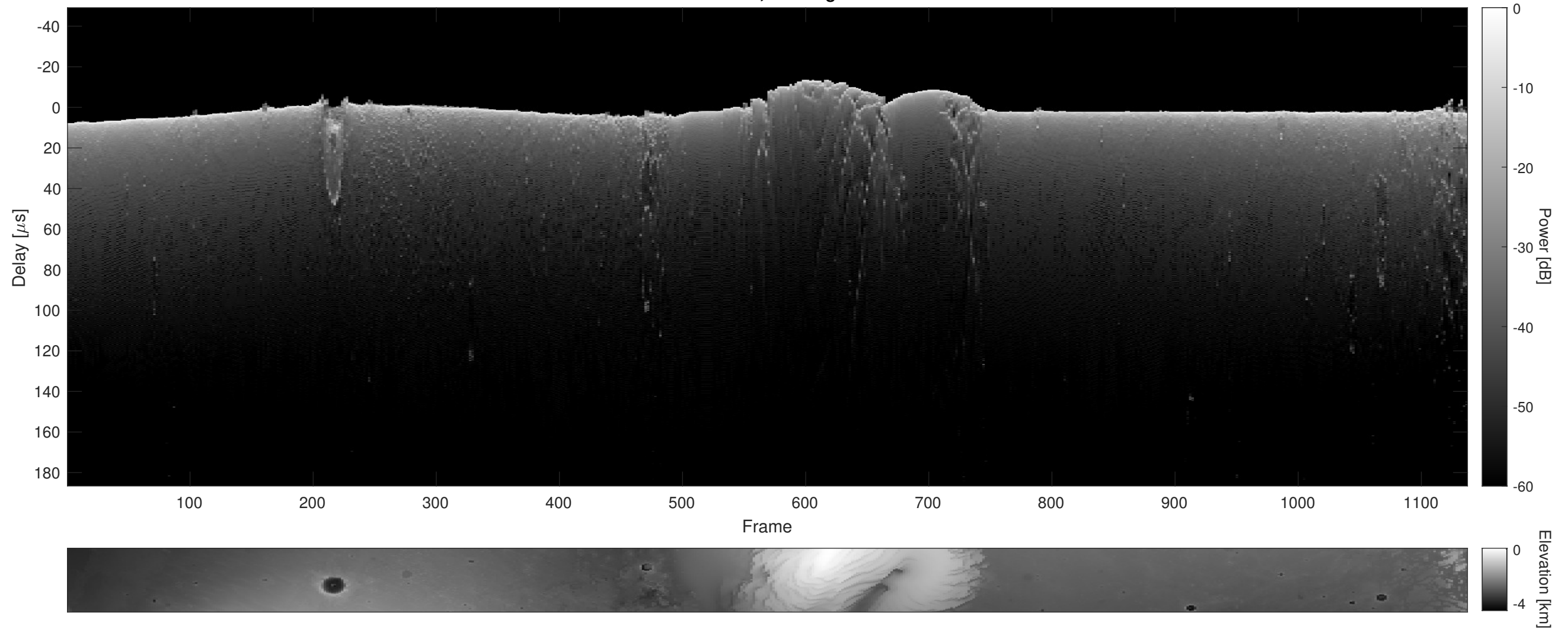
Orbit 11910, Cluttergram
