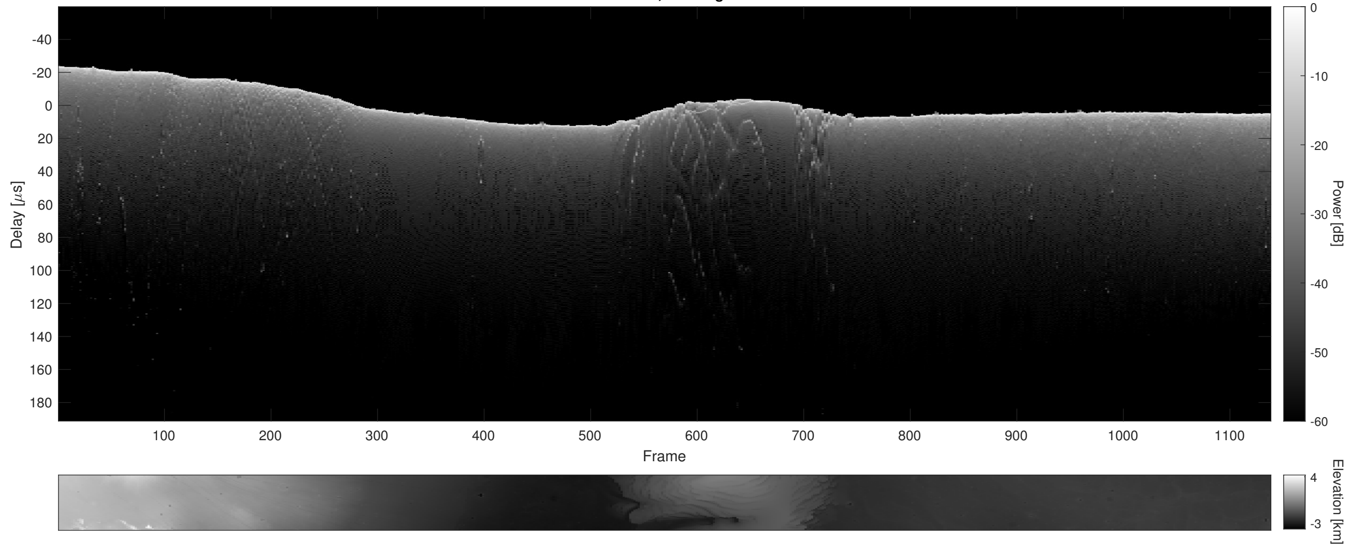
Orbit 11913, Cluttergram
