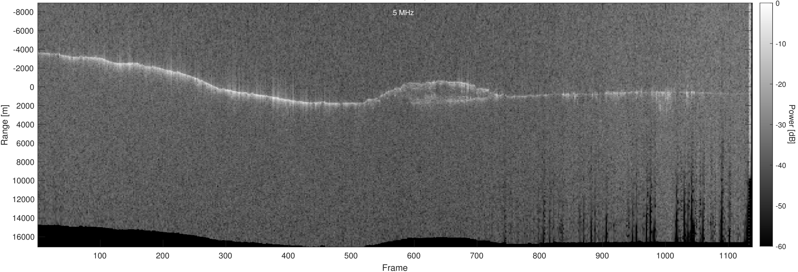
Orbit 11913, Optimized, No Window, Depth-Corrected, Channel 2
