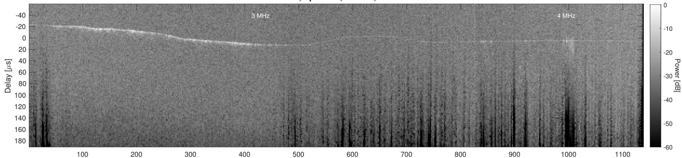
Orbit 11913, Cluttergram
