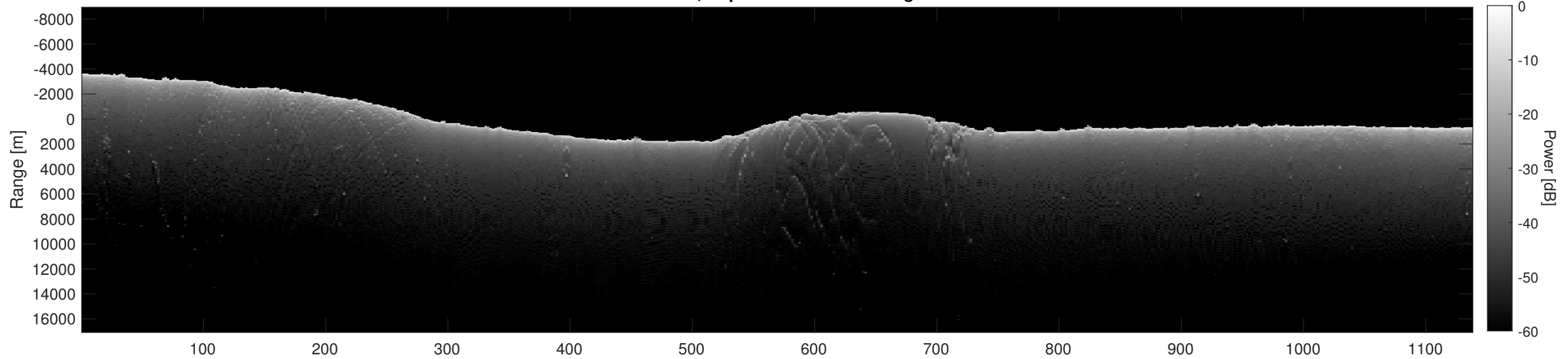
Orbit 11913, Depth-Corrected Cluttergram
