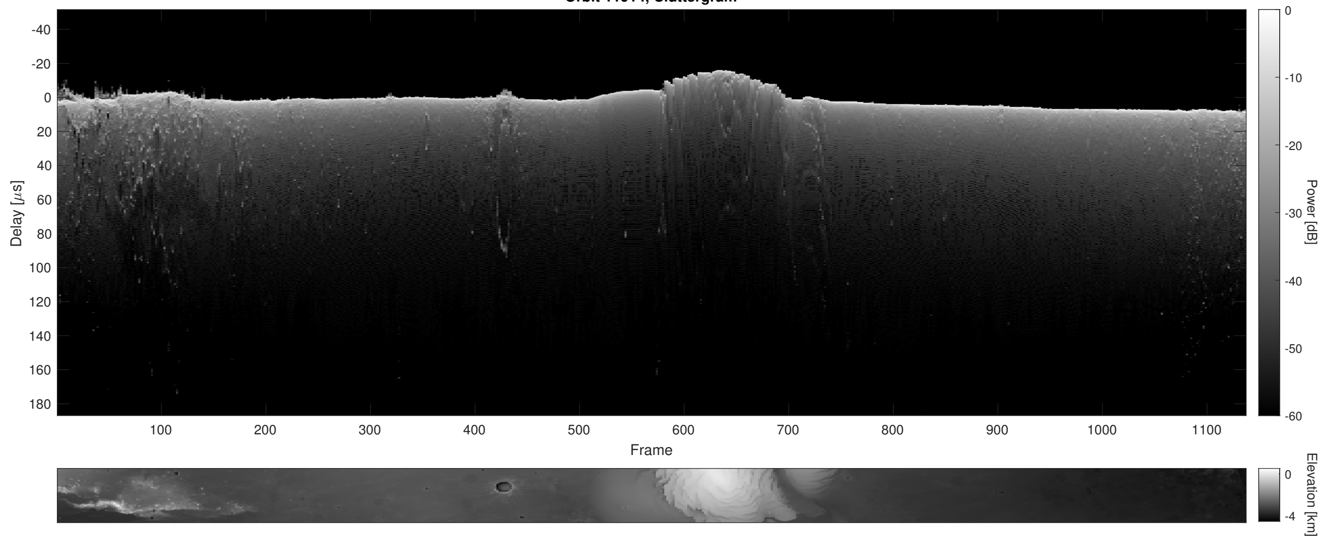
Orbit 11914, Cluttergram
