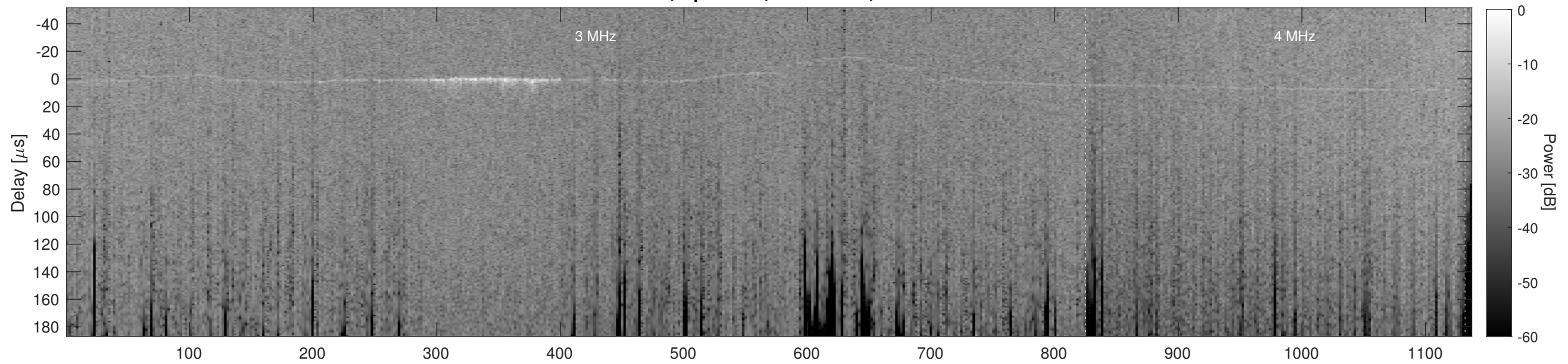
Orbit 11914, Cluttergram
