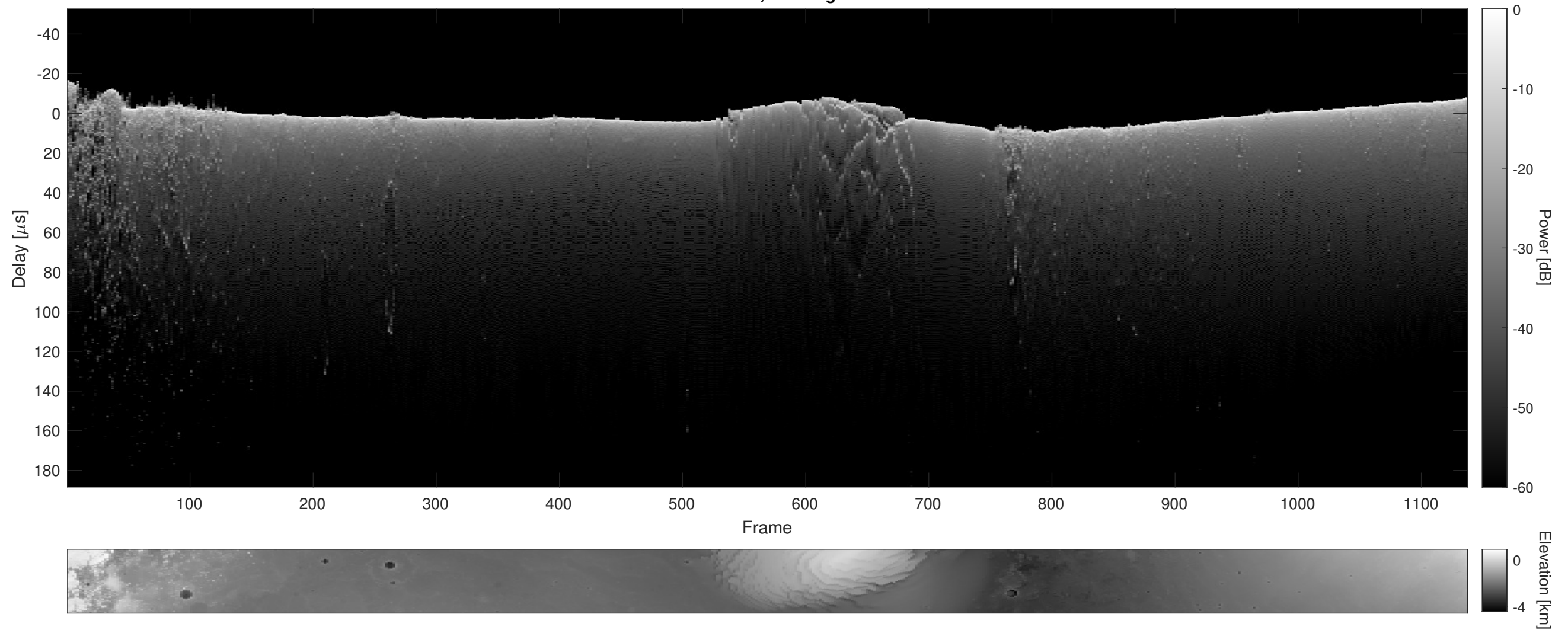
Orbit 11915, Cluttergram
