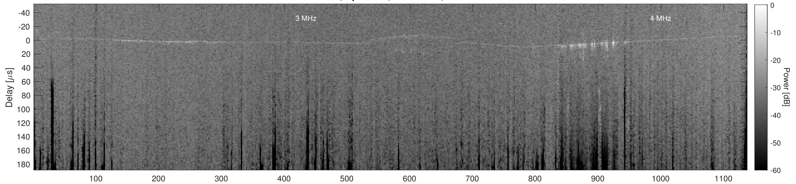
Orbit 11915, Cluttergram
