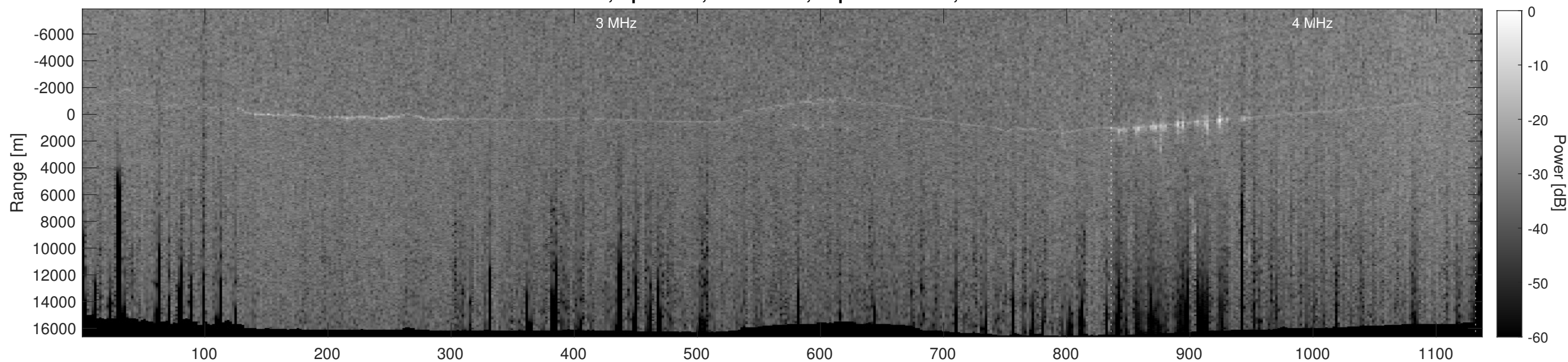
Orbit 11915, Depth-Corrected Cluttergram
