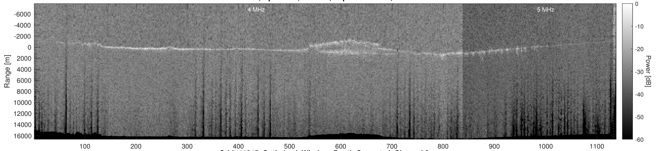
Orbit 11915, Optimized, Window, Depth-Corrected, Channel 2
