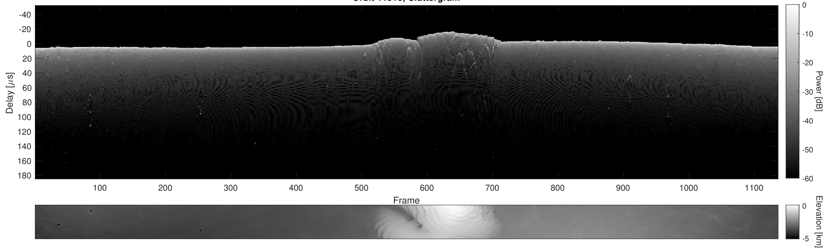
Orbit 11916, Cluttergram
