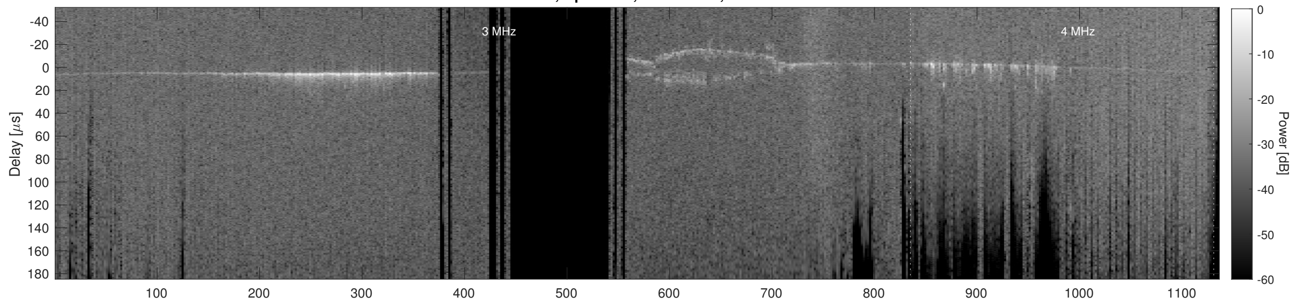
Orbit 11916, Cluttergram
