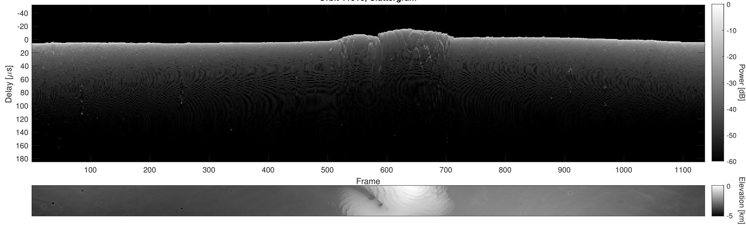
Orbit 11916, Cluttergram
