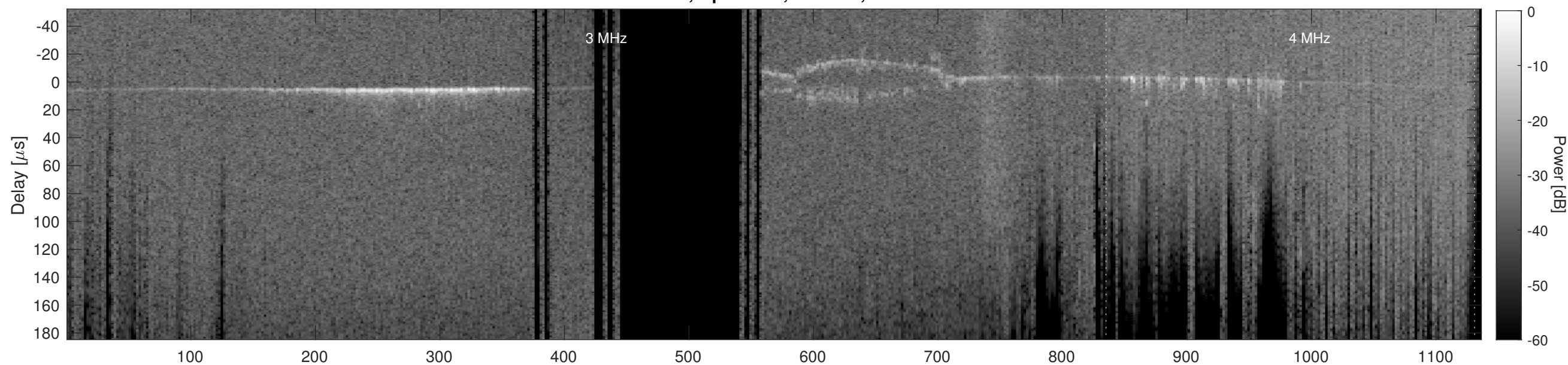
Orbit 11916, Cluttergram
