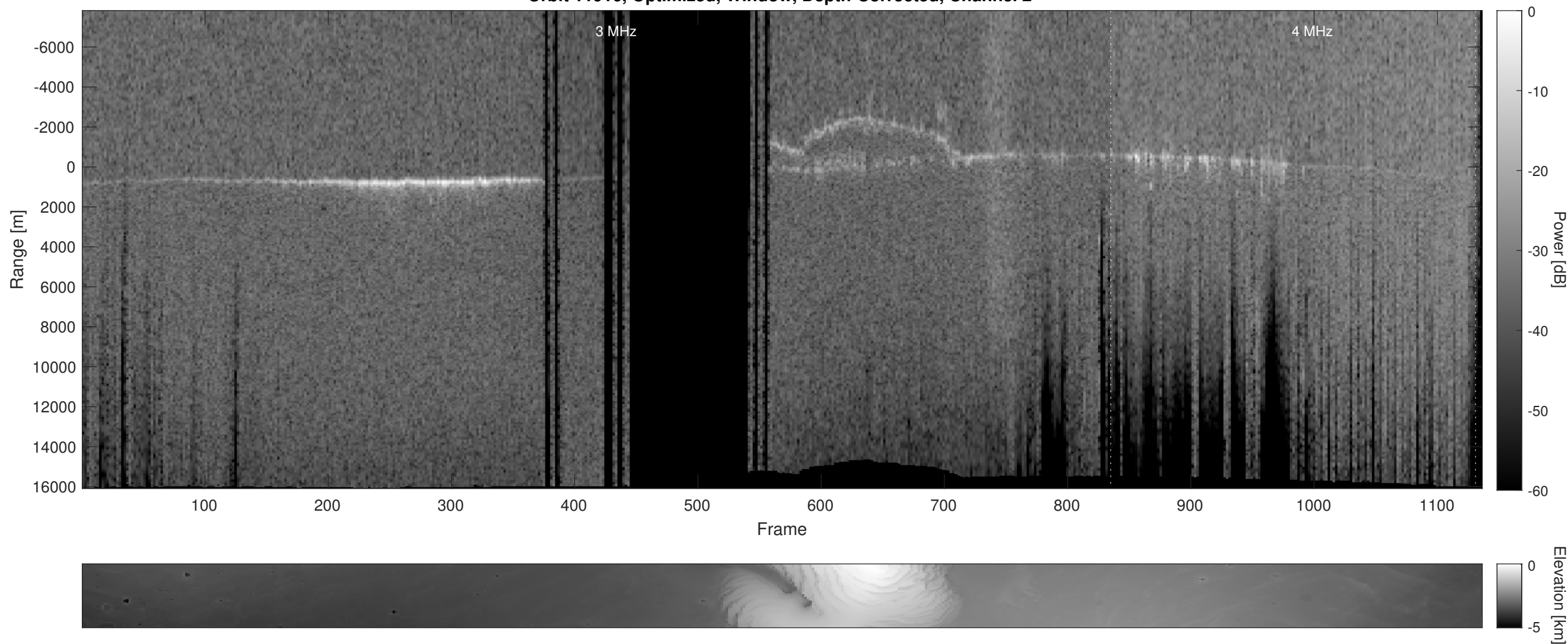
Orbit 11916, Optimized, Window, Depth-Corrected, Channel 2
