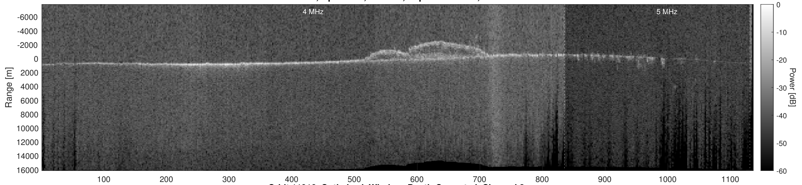
Orbit 11916, Optimized, Window, Depth-Corrected, Channel 2
