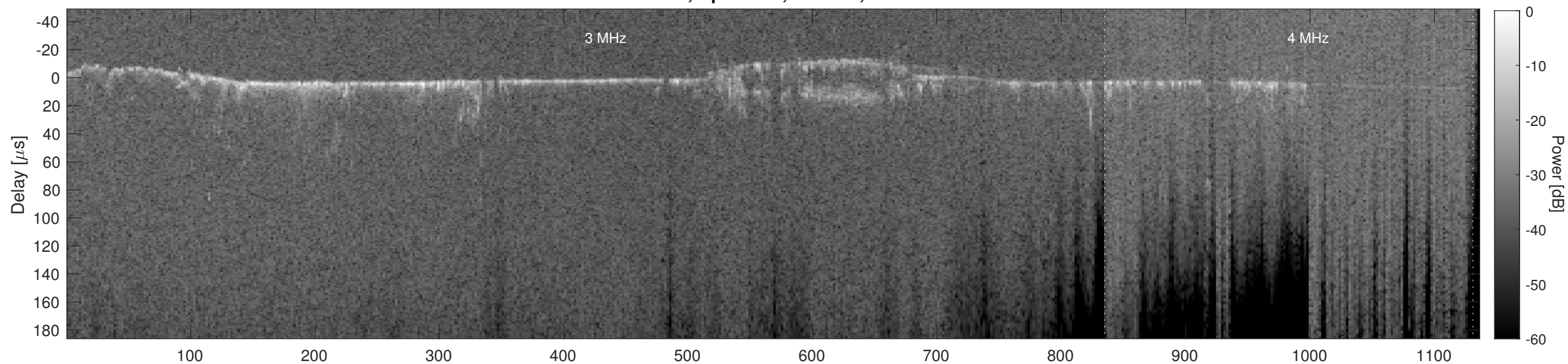
Orbit 11919, Cluttergram
