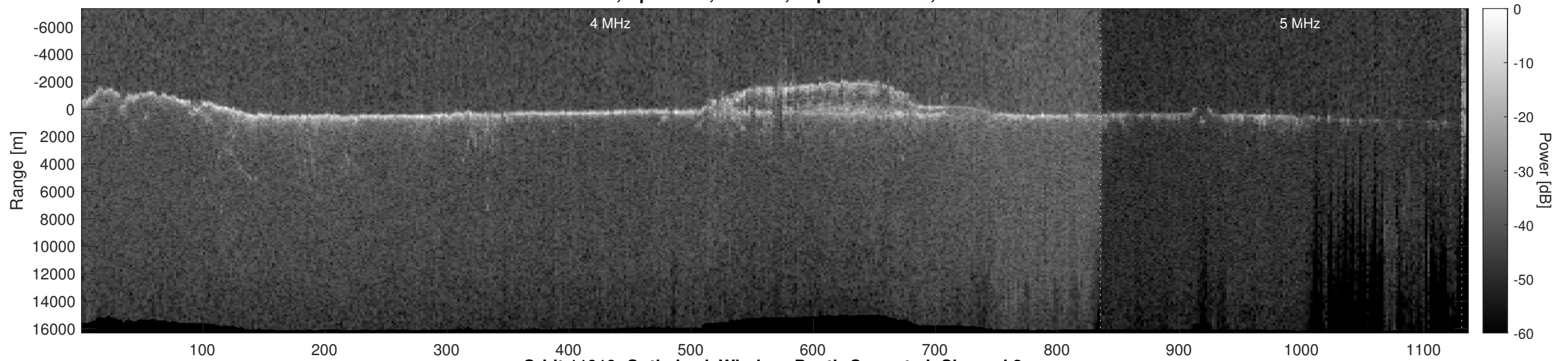
Orbit 11919, Optimized, Window, Depth-Corrected, Channel 2
