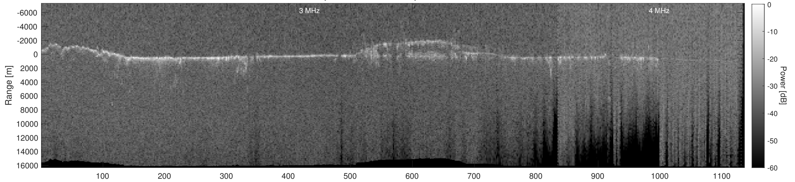
Orbit 11919, Depth-Corrected Cluttergram
