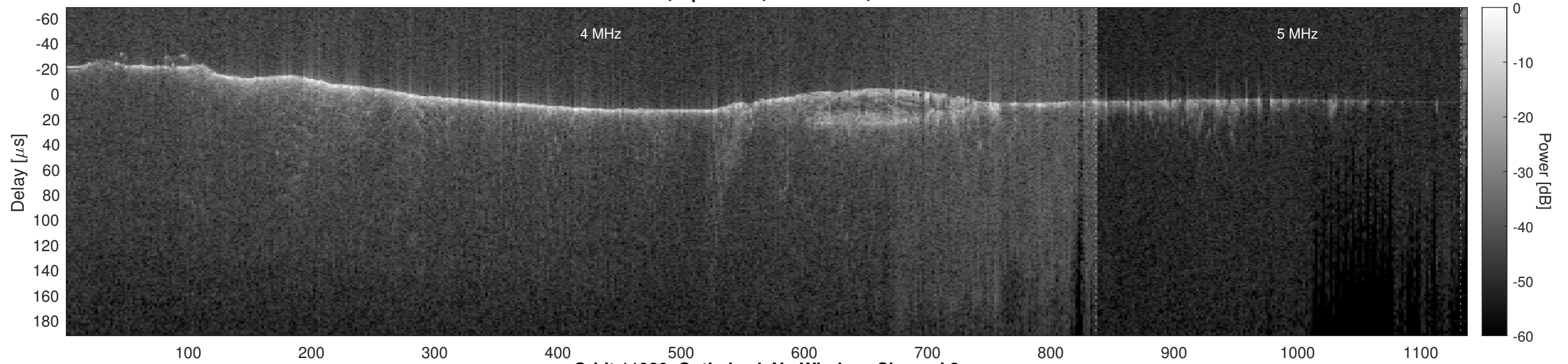
Orbit 11920, Optimized, No Window, Channel 2
