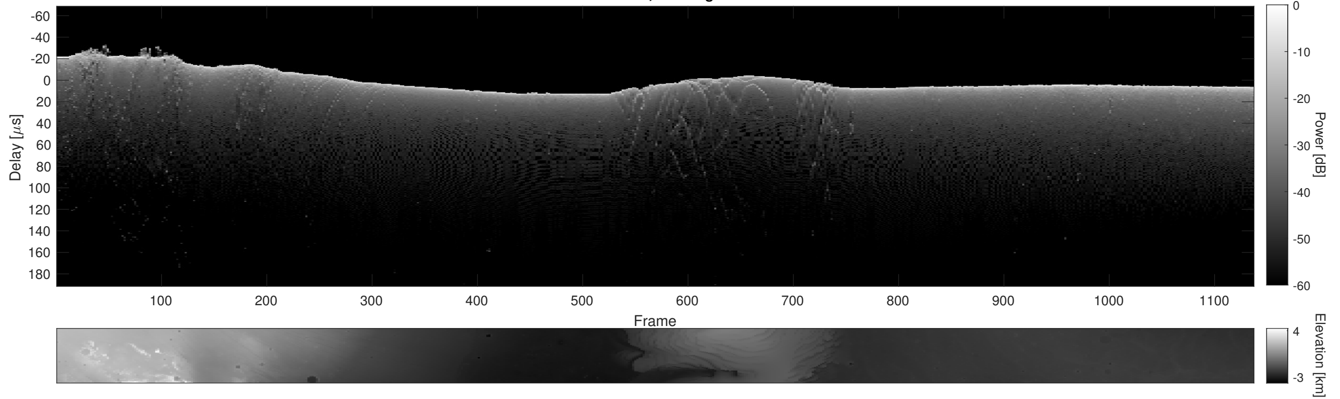
Orbit 11920, Cluttergram
