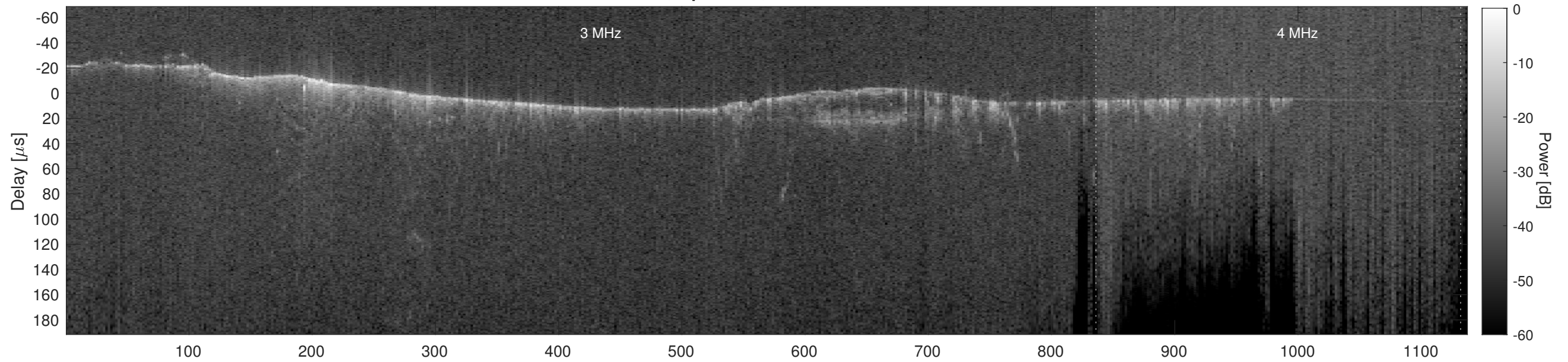
Orbit 11920, Cluttergram
