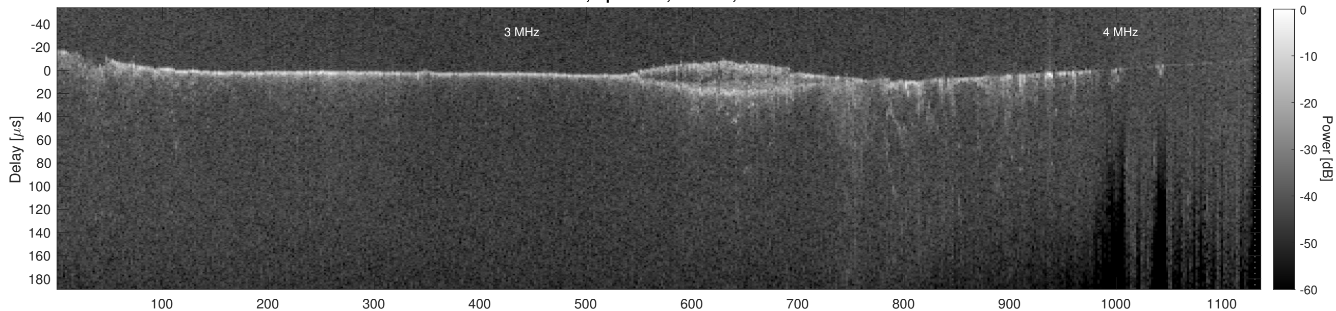
Orbit 11922, Cluttergram
