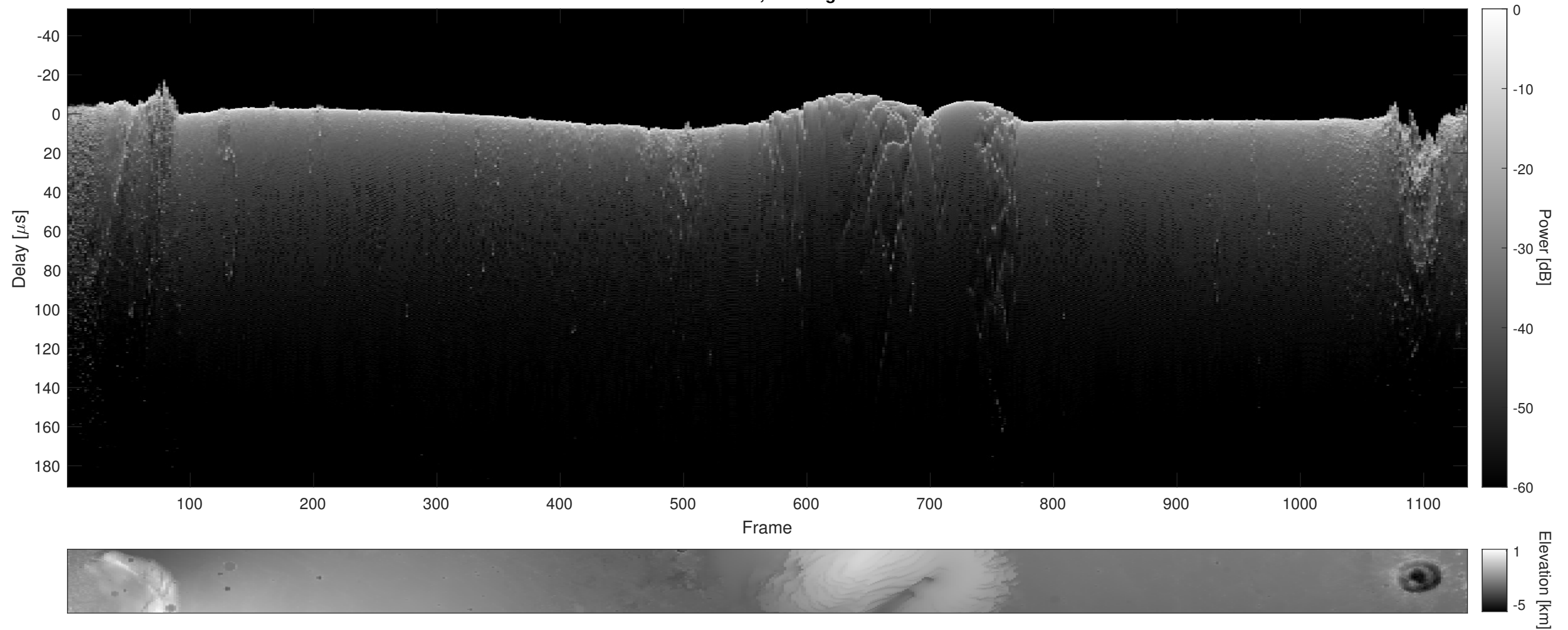
Orbit 11924, Cluttergram
