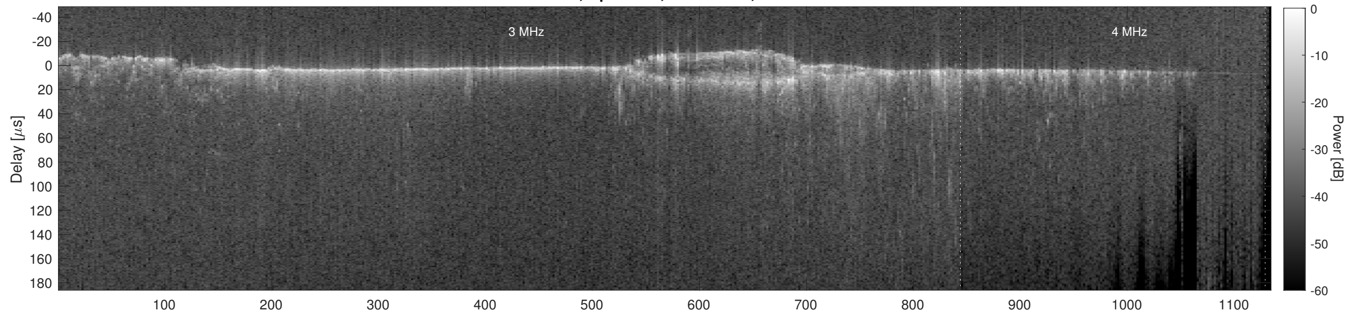
Orbit 11926, Cluttergram
