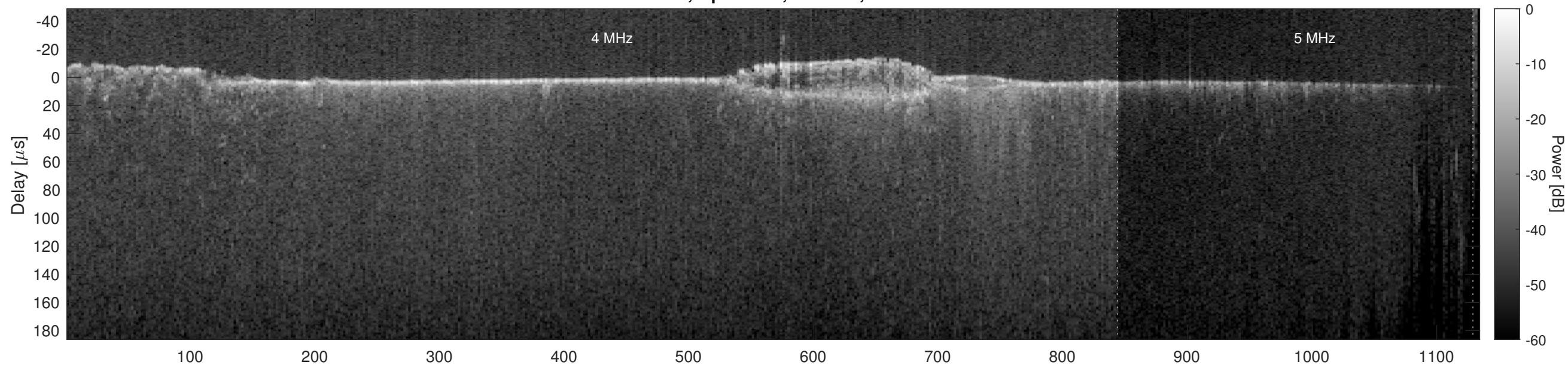
Orbit 11926, Optimized, Window, Channel 2
