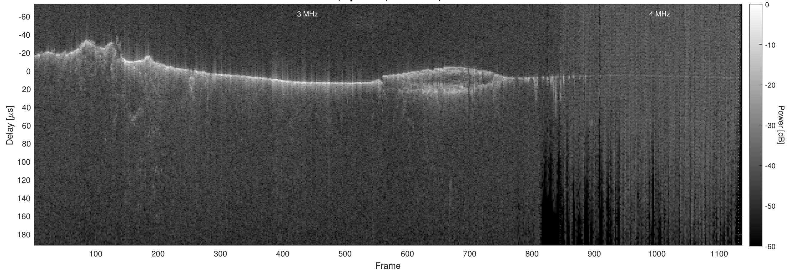
Orbit 11927, Optimized, No Window, Channel 2
