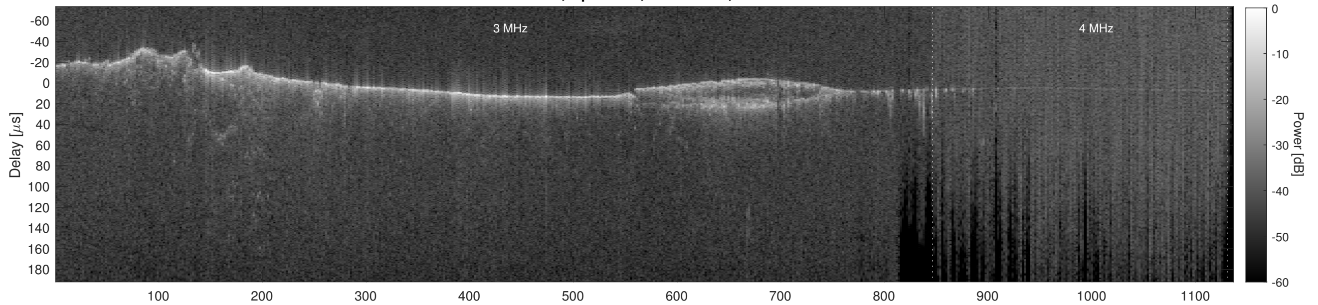
Orbit 11927, Cluttergram
