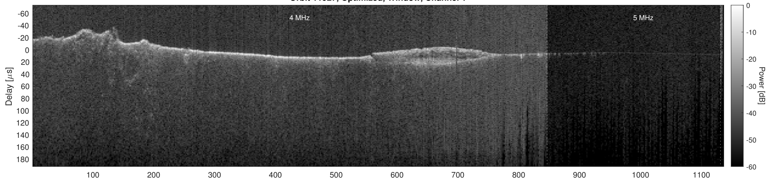
Orbit 11927, Optimized, Window, Channel 2
