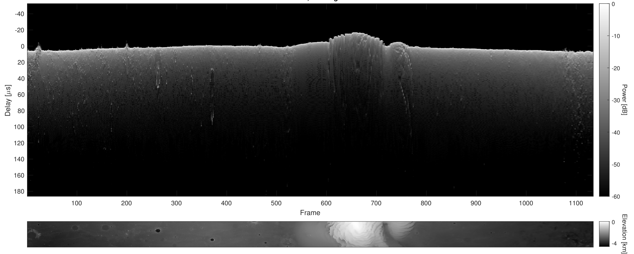
Orbit 11928, Cluttergram
