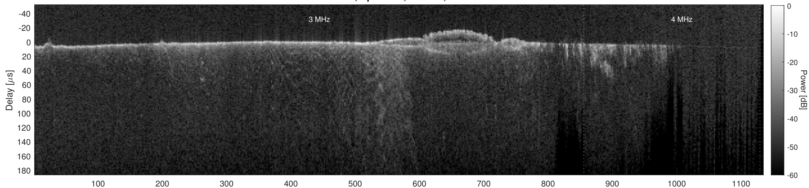
Orbit 11928, Cluttergram
