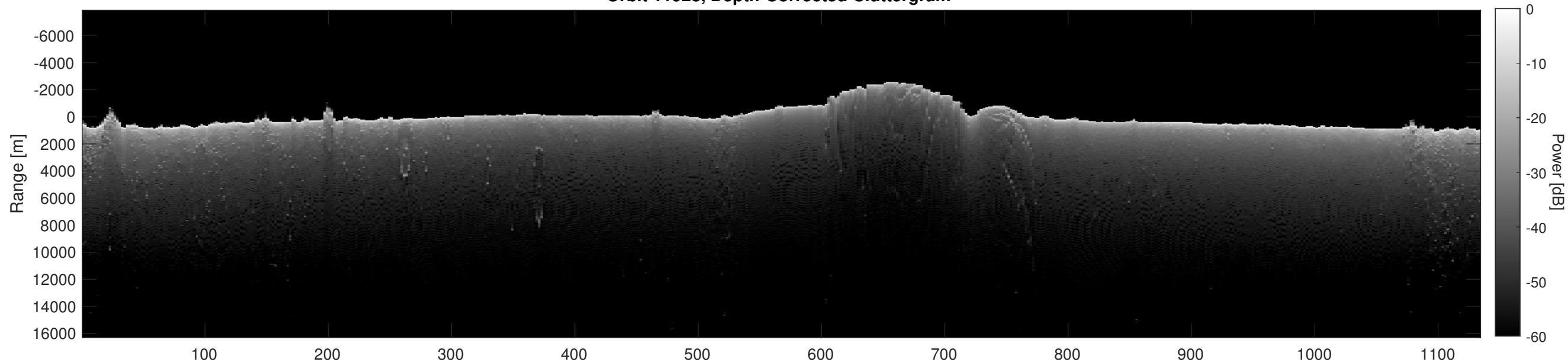
Orbit 11928, Depth-Corrected Cluttergram
