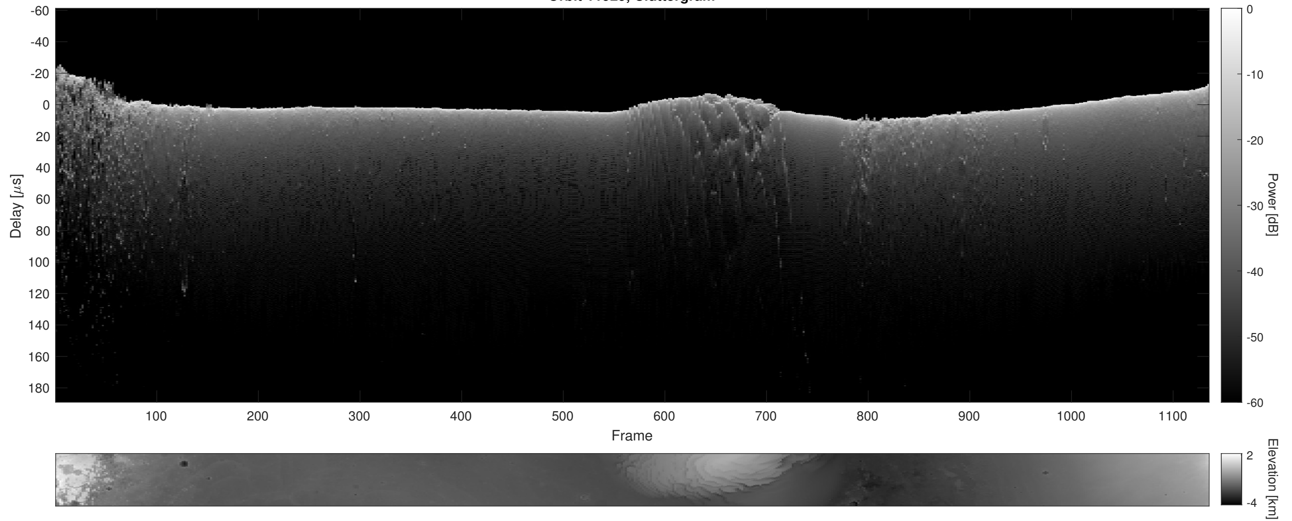
Orbit 11929, Cluttergram
