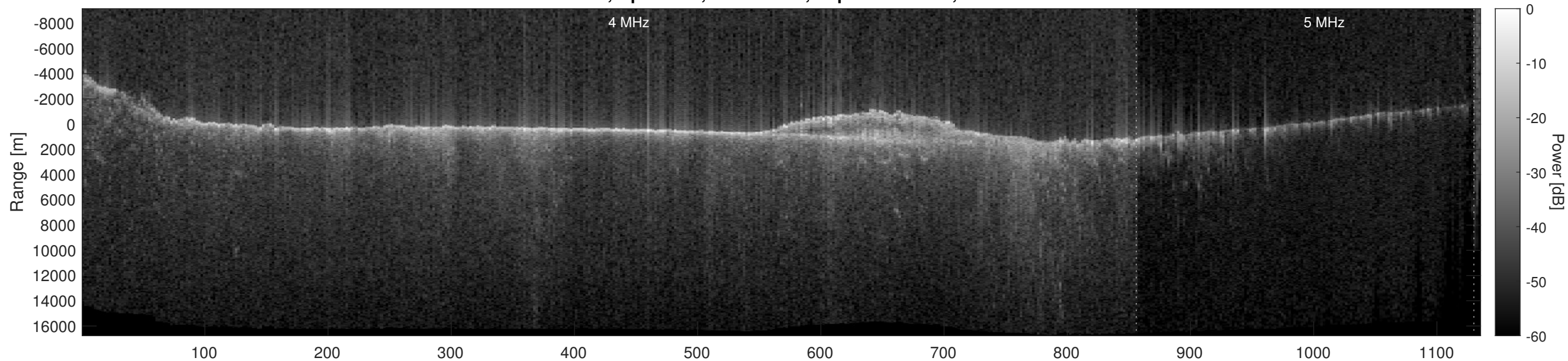
Orbit 11929, Optimized, No Window, Depth-Corrected, Channel 2
