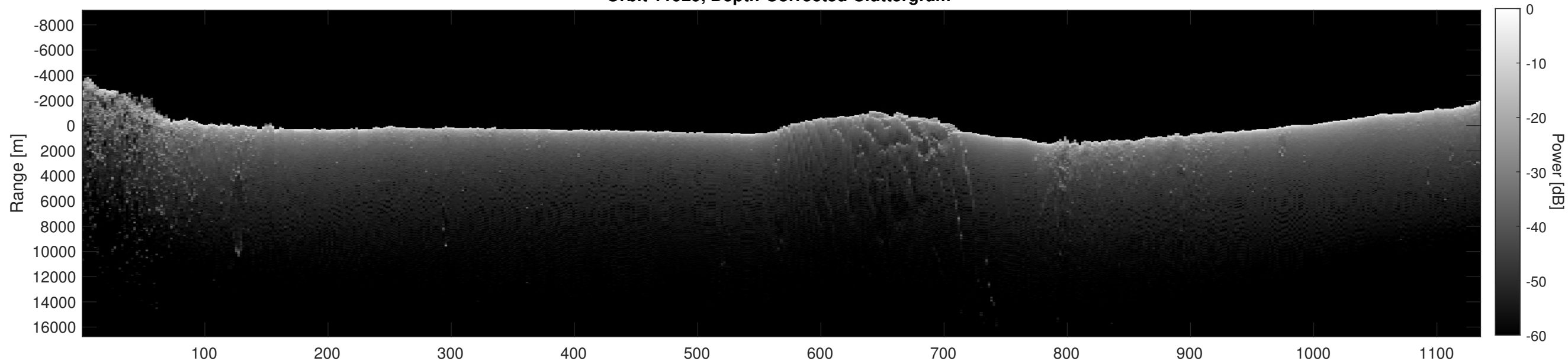
Orbit 11929, Depth-Corrected Cluttergram
