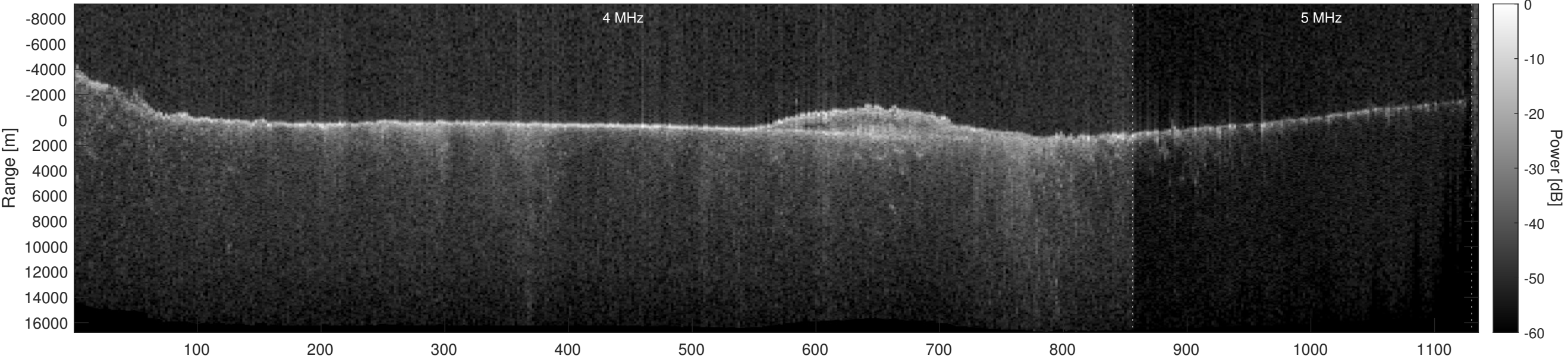
Orbit 11929, Optimized, Window, Depth-Corrected, Channel 2
