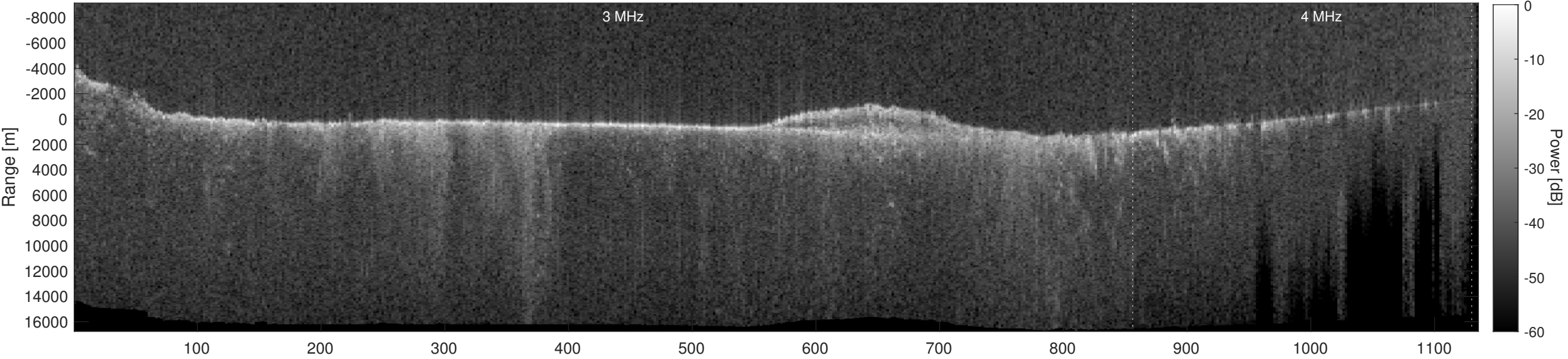
Orbit 11929, Depth-Corrected Cluttergram
