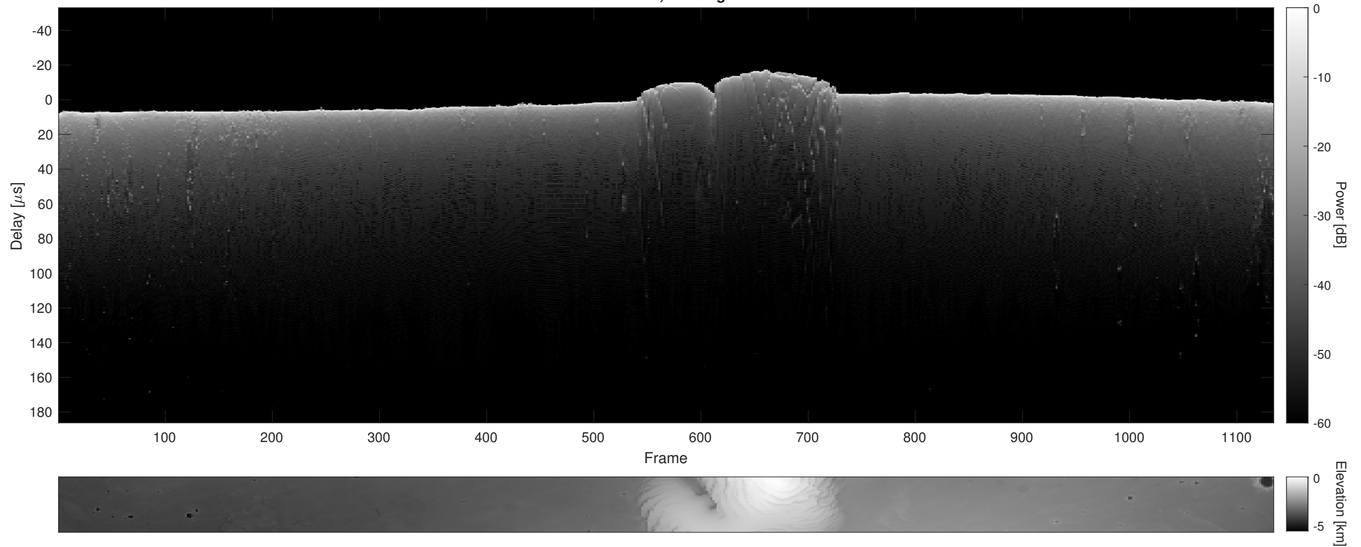
Orbit 11930, Cluttergram
