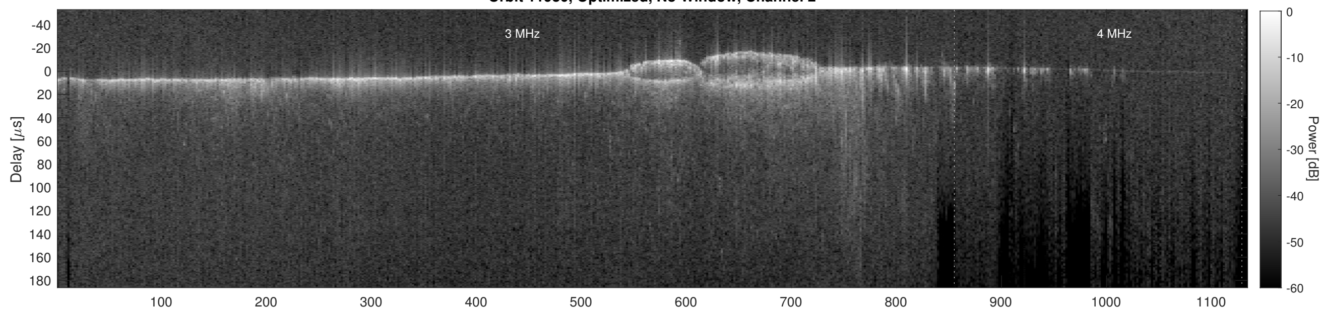
Orbit 11930, Cluttergram
