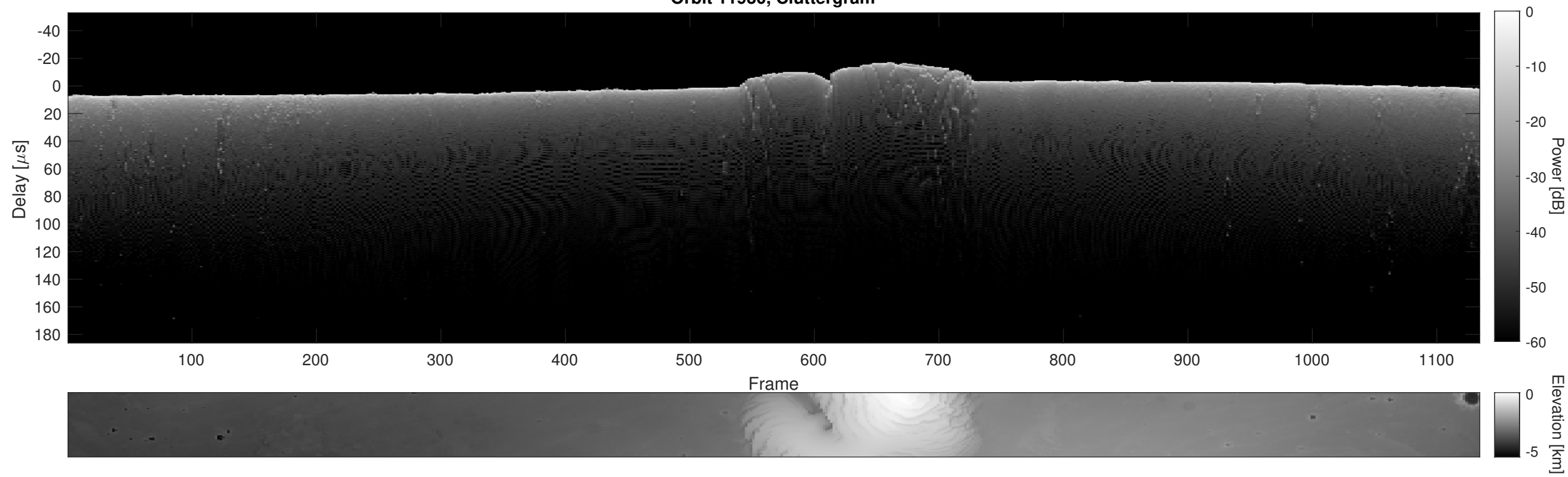
Orbit 11930, Cluttergram
