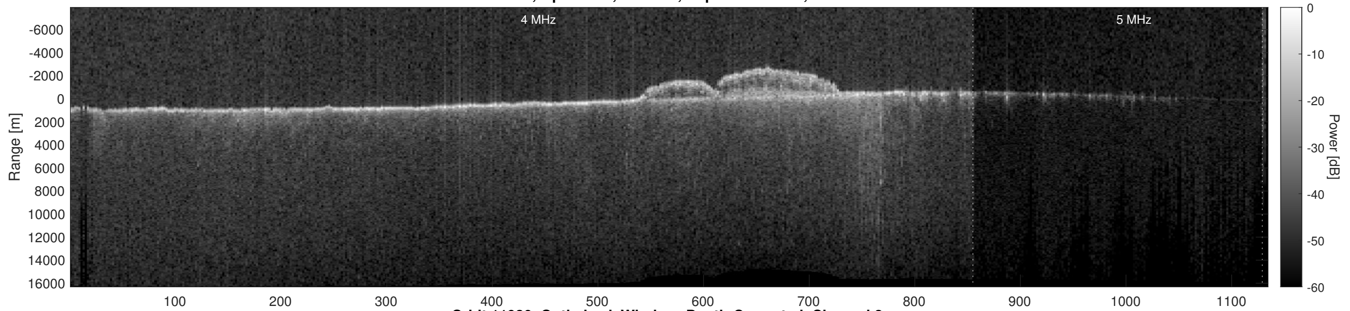
Orbit 11930, Optimized, Window, Depth-Corrected, Channel 2
