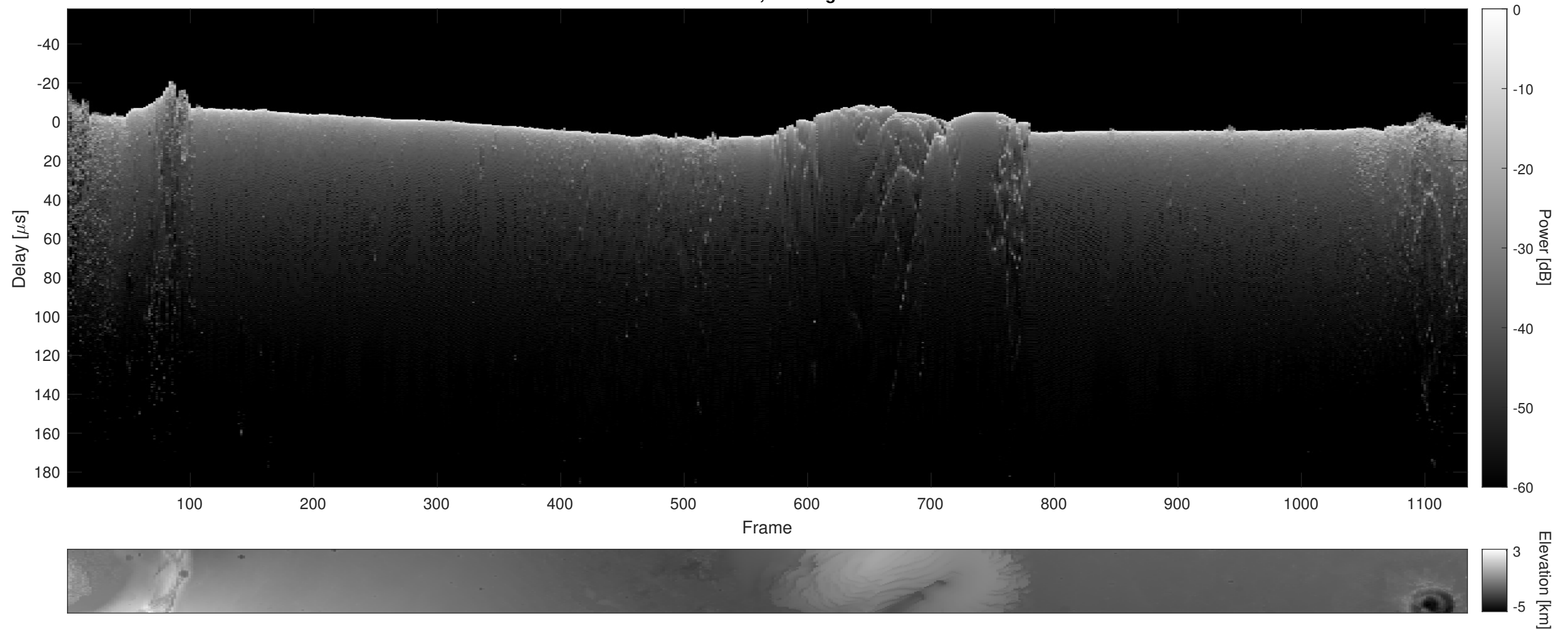
Orbit 11931, Cluttergram
