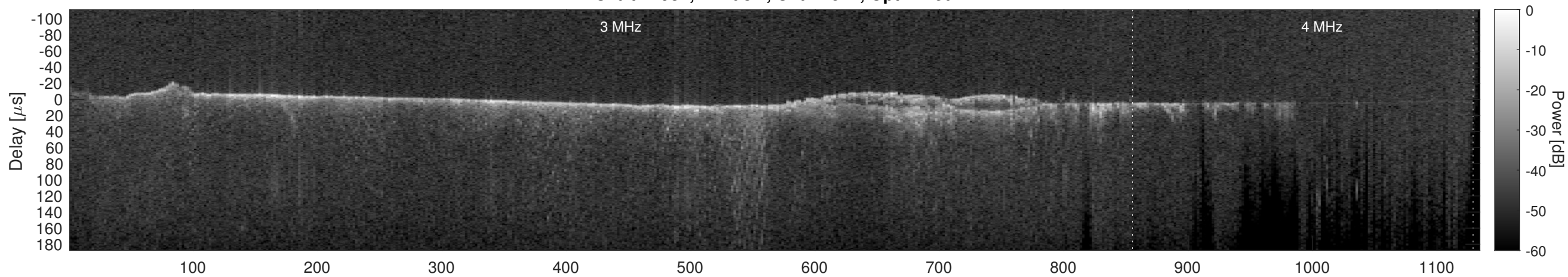
Orbit 11931, Cluttergram
