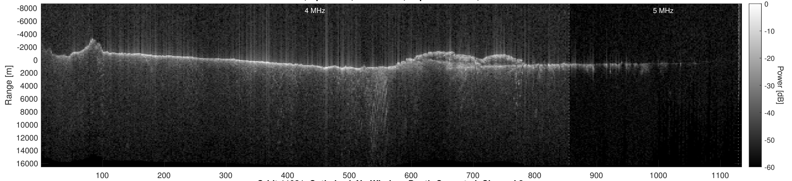
Orbit 11931, Optimized, No Window, Depth-Corrected, Channel 2
