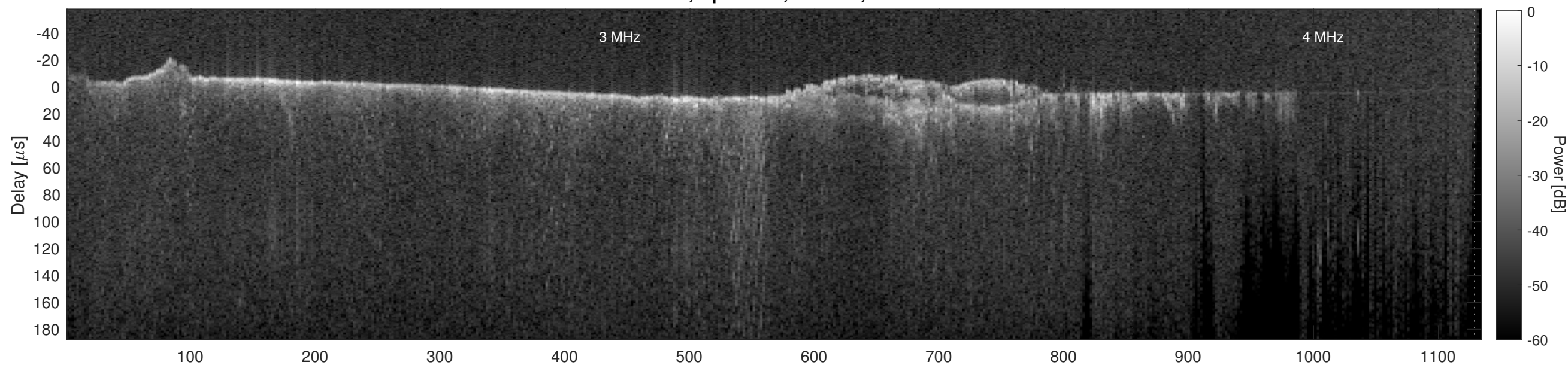
Orbit 11931, Cluttergram
