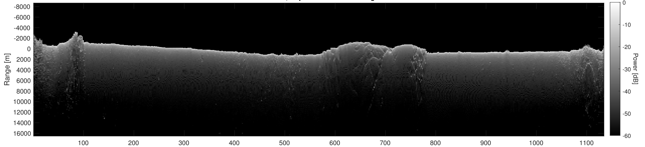
Orbit 11931, Depth-Corrected Cluttergram
