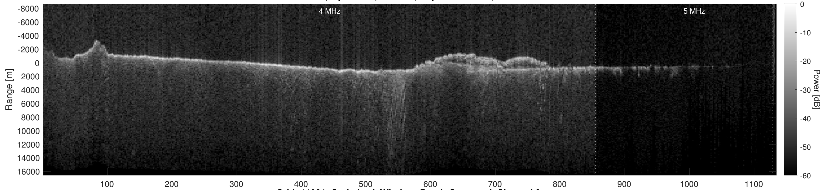
Orbit 11931, Optimized, Window, Depth-Corrected, Channel 2
