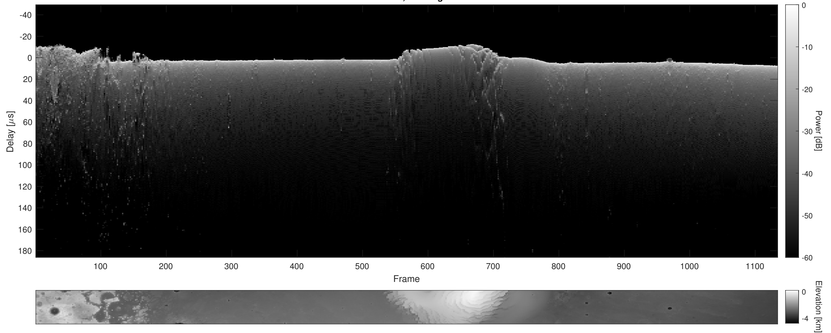
Orbit 11933, Cluttergram
