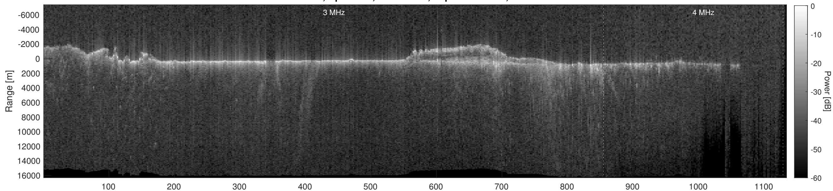
Orbit 11933, Depth-Corrected Cluttergram
