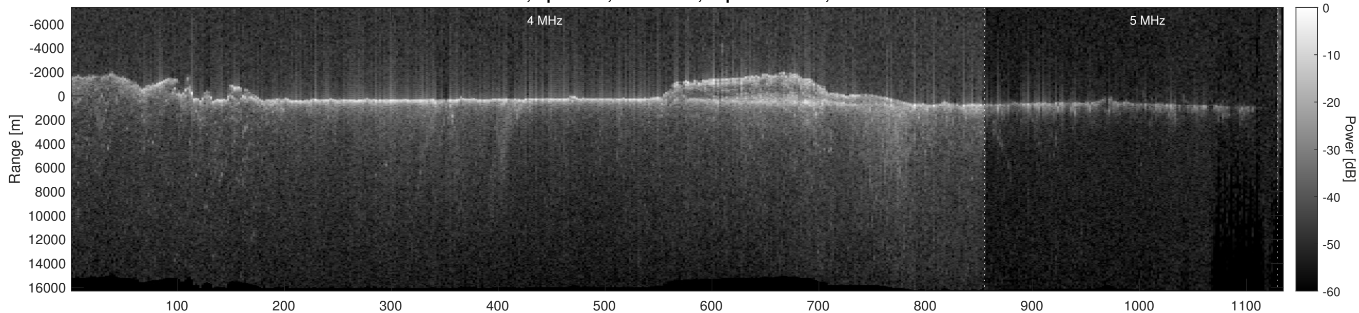
Orbit 11933, Optimized, No Window, Depth-Corrected, Channel 2
