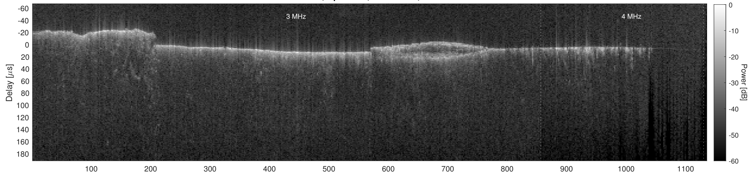
Orbit 11934, Cluttergram
