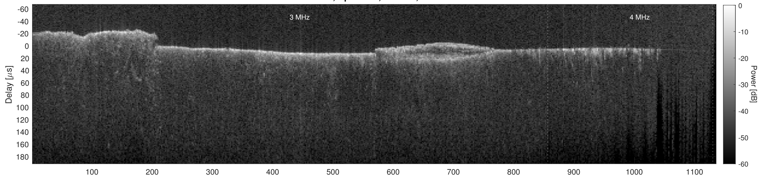
Orbit 11934, Cluttergram
