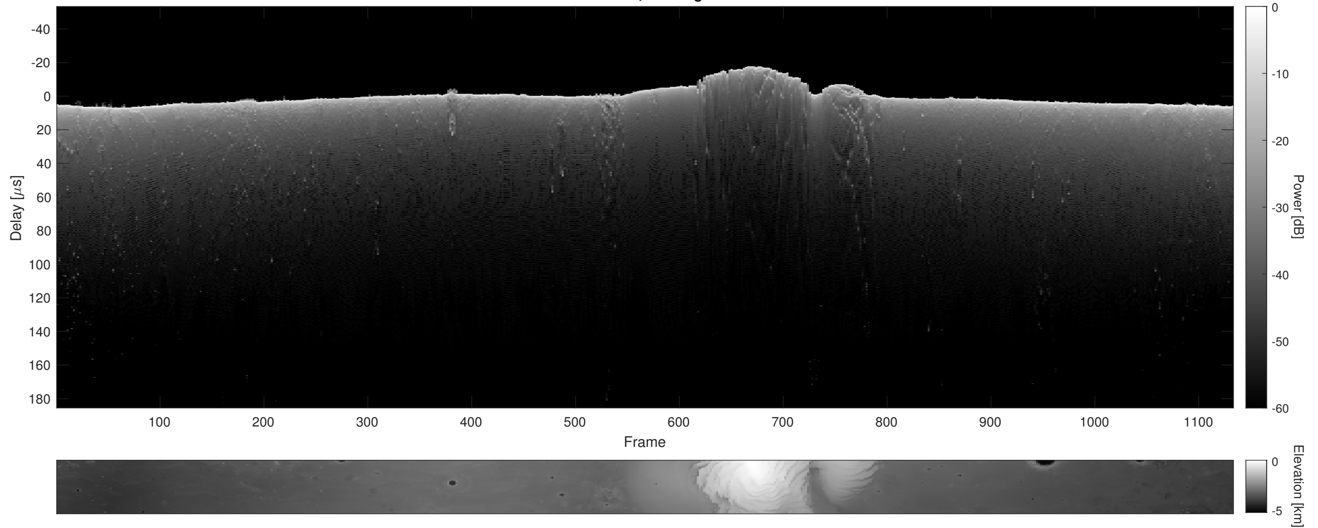
Orbit 11935, Cluttergram
