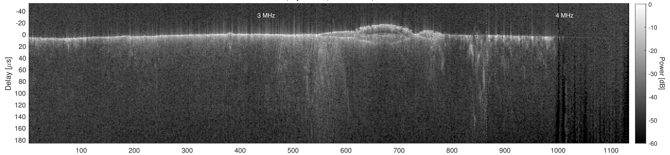
Orbit 11935, Cluttergram
